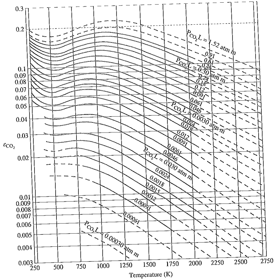
Figure Emissivity of carbon dioxide at a total pressure of 1 atm
