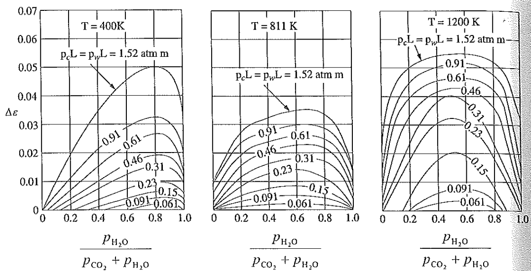
Figure Factor \Delta \epsilon to correct the emissivity of a mixture of water vapor and \text{CO}_2
