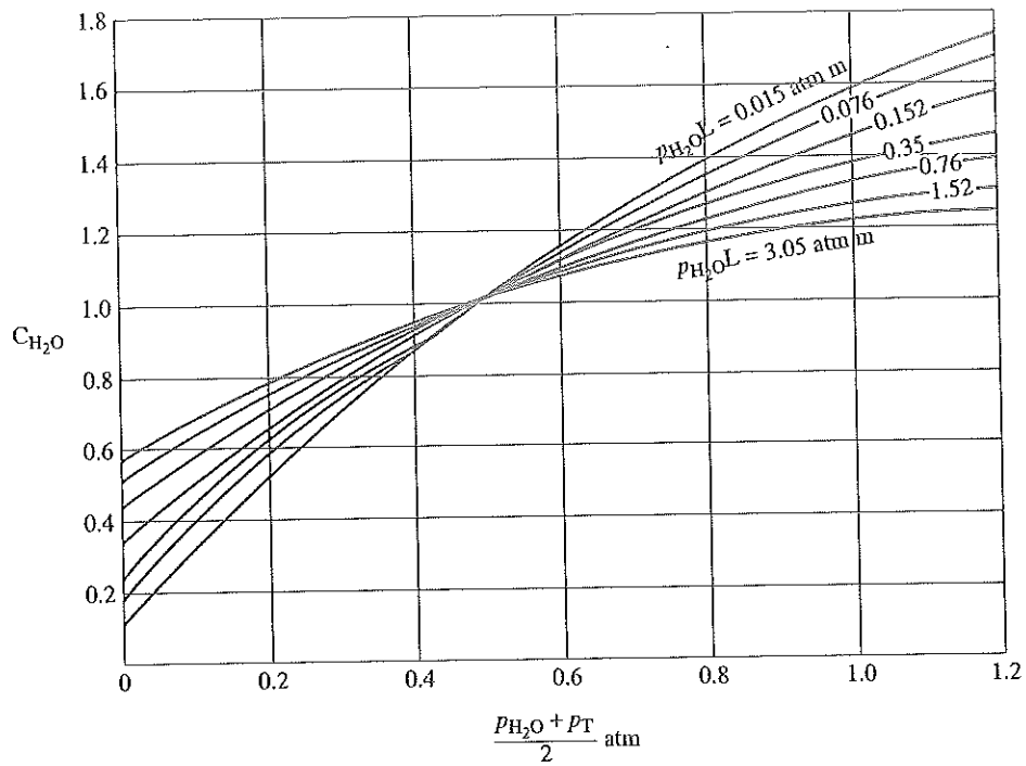
Figure Correction factor for the emissivity of water vapor at pressures other than 1 atm
