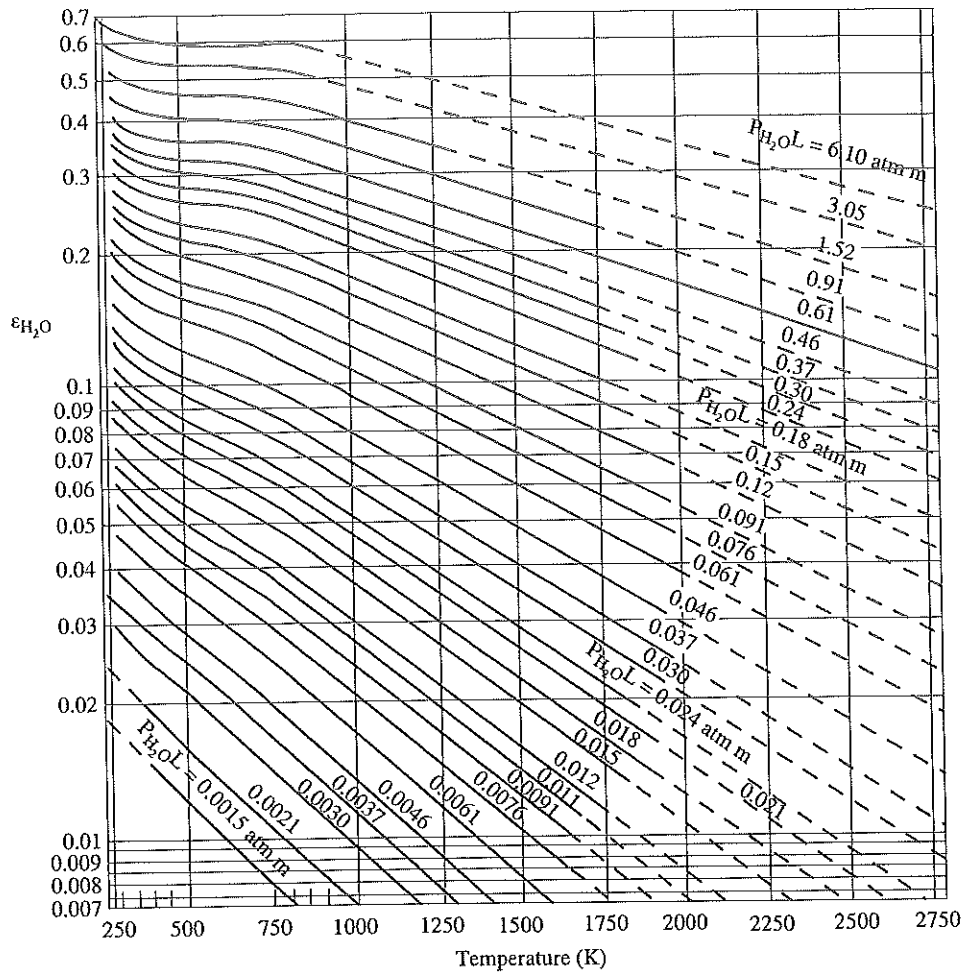
Figure 13.54 Emissivity of water vapor at a total pressure of 1 atm
