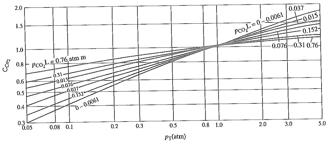
Figure Correction factor for the emissivity of carbon dioxide at pressures other than 1 atm
